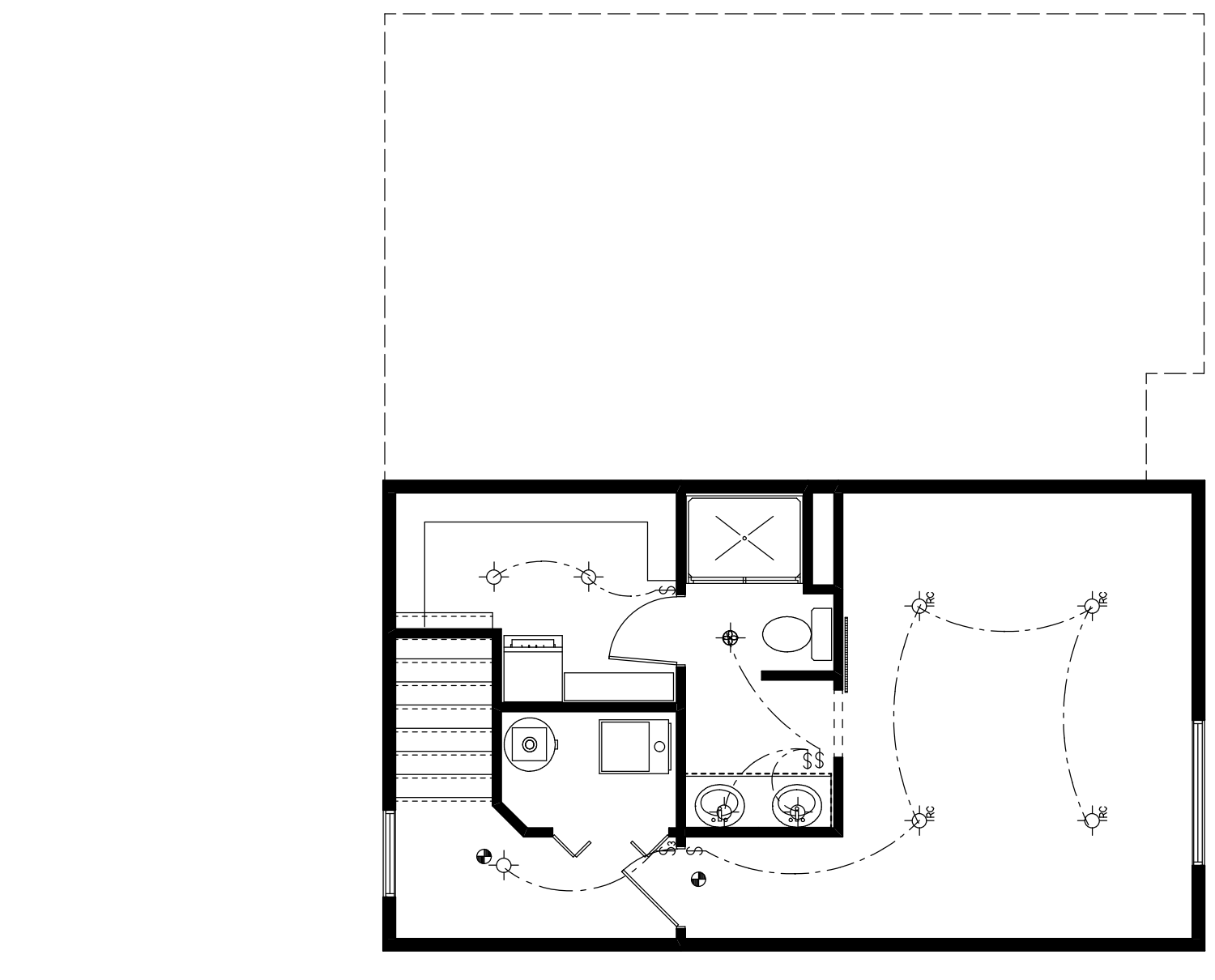
UPPER FLOOR ELECTRICAL PLAN
