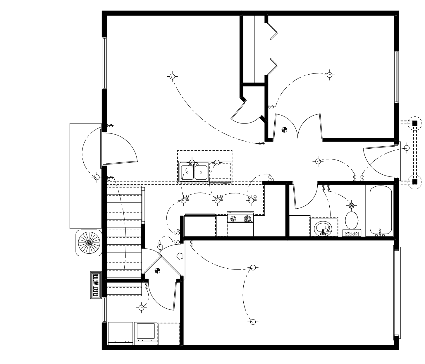
GROUND FLOOR ELECTRICAL PLAN
