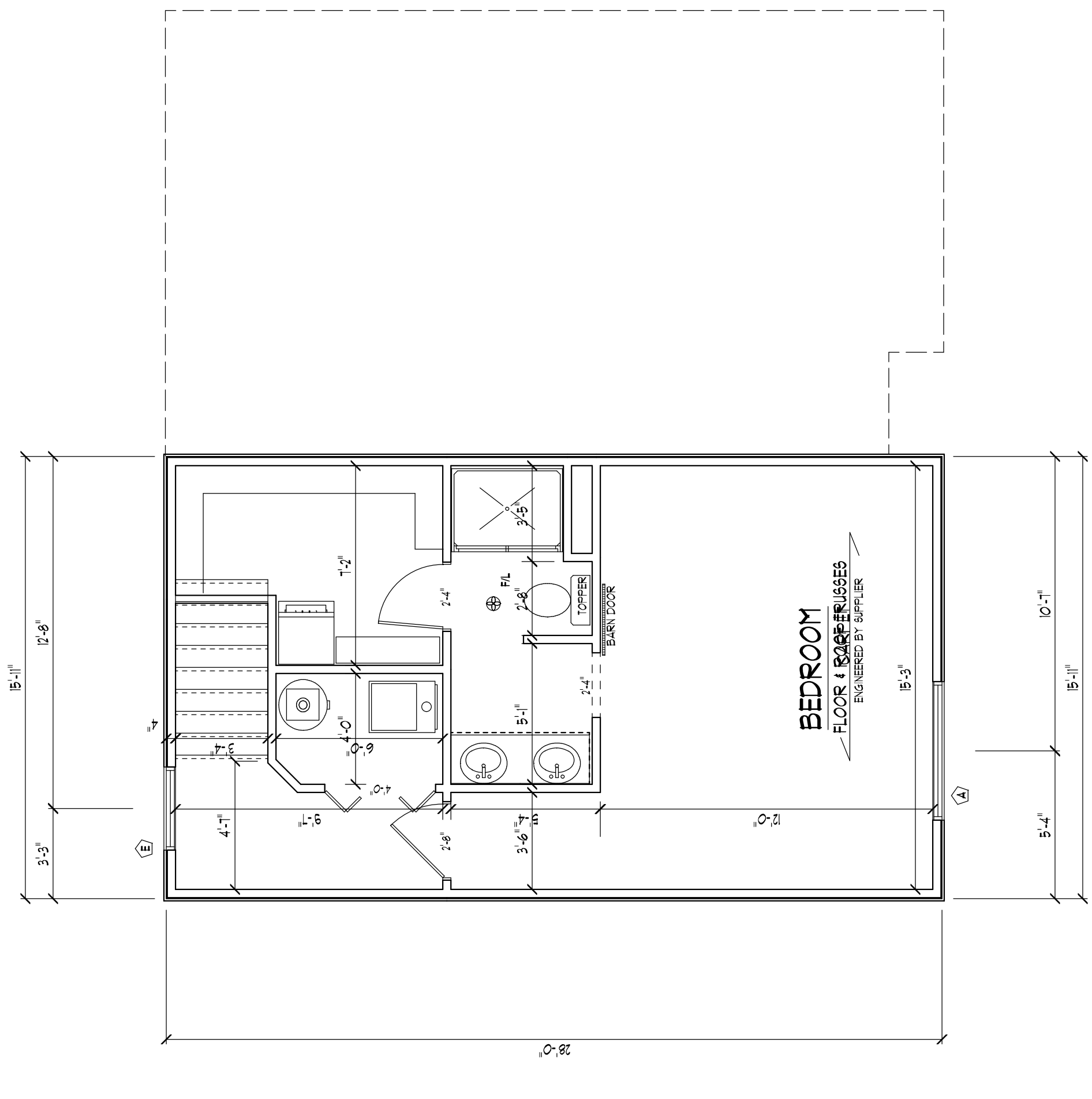
UPPER FLOOR PLAN SCALE: 1/4" = 1'-0"
