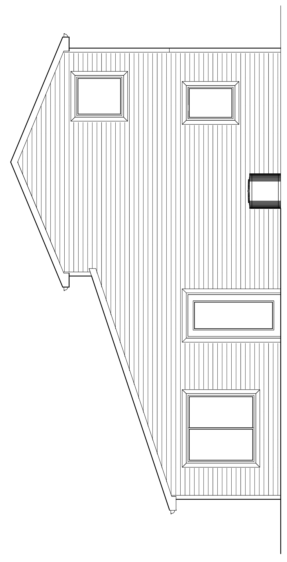
REAR ELEVATION SCALE: 1/4" = 1'-0"
